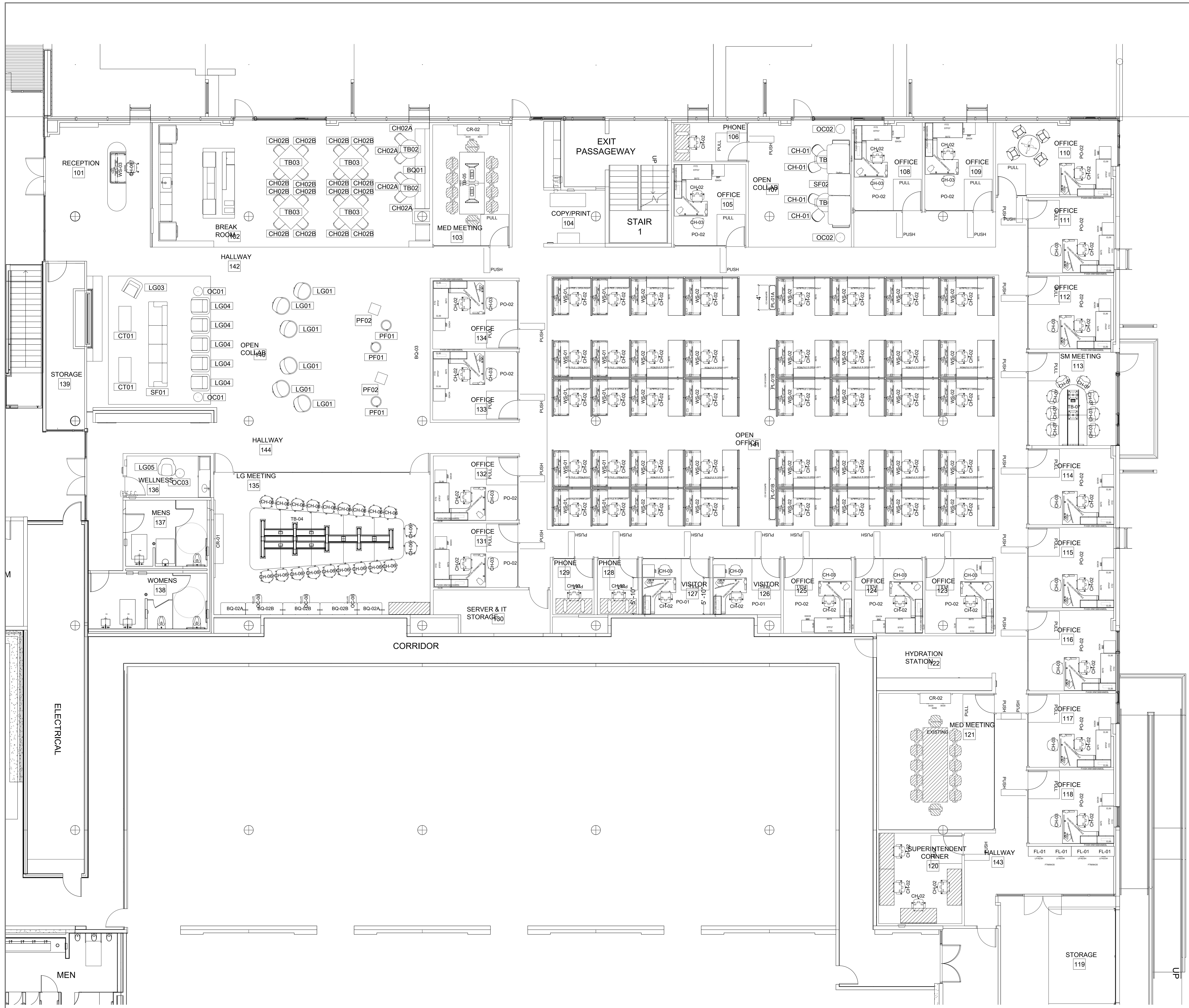
PLAN VIEW
